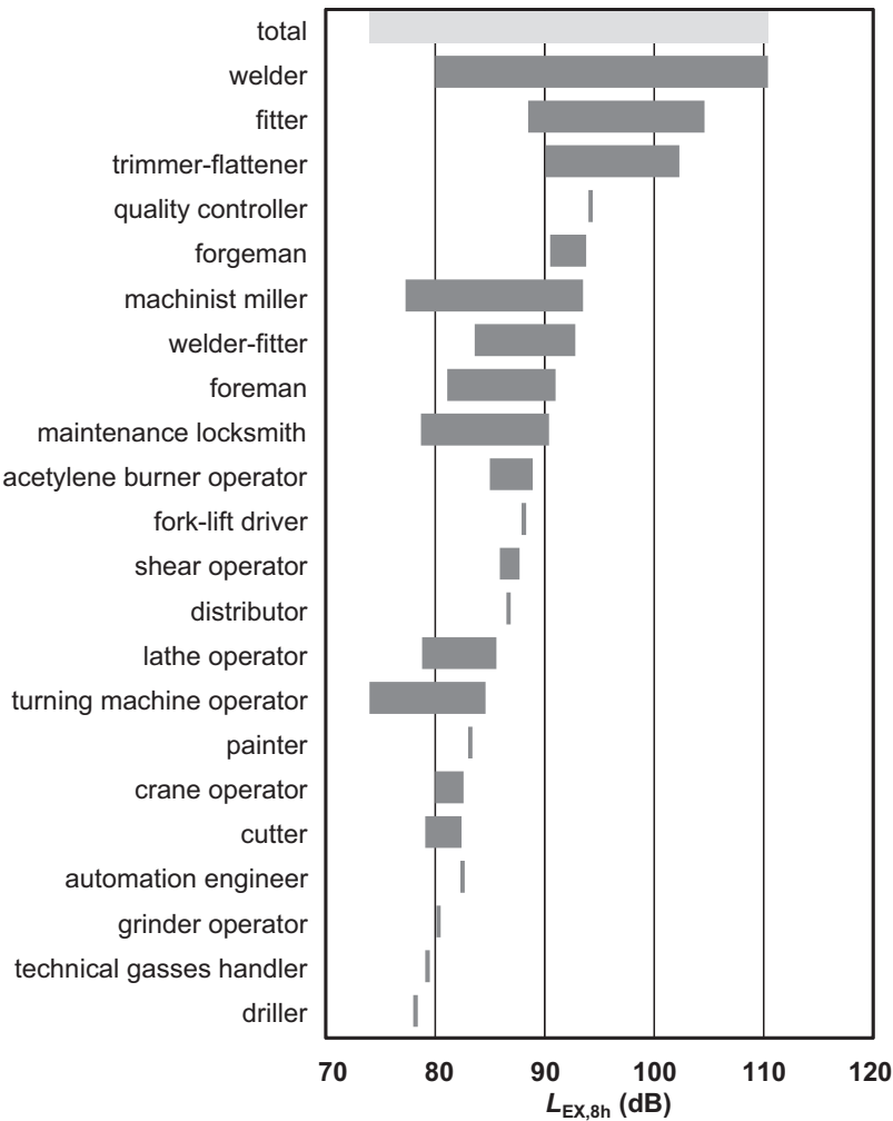
Figure 1. Daily noise exposure levels ( L_{EX,8h} ) determined for various workstations (each bar represents a range from minimum to maximum values).
