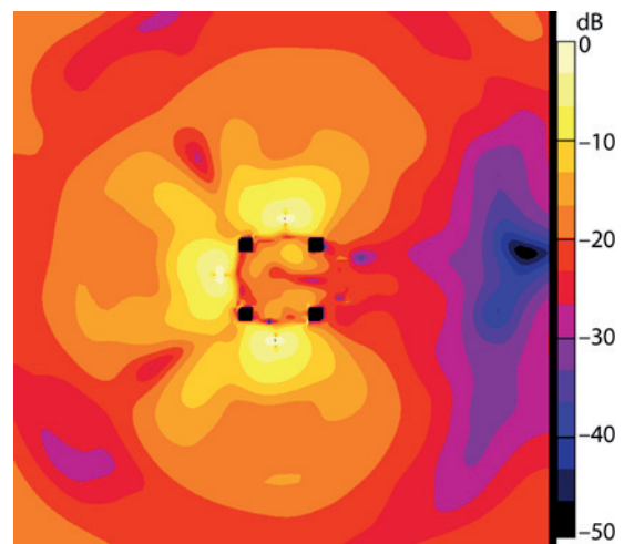
Figure 3. Electric field strength in a horizontal cross-section. Notes. The results are normalized to 1000 V/m and shown in logarithmic scale.
