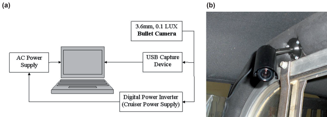
Figure 1. In-car video collection system (a) components and layout, and (b) camera placement on the passenger-side roll cage of police cruiser.
