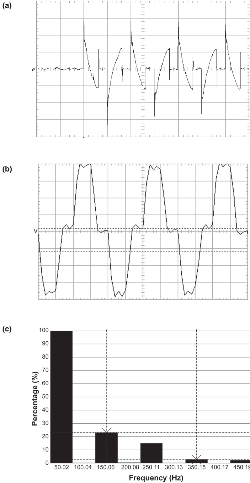
Figure 1. Magnetic field from a spot welding machine: (a) time derivative dB/dt recorded with a small pick up coil, 10 ms/div; (b) magnetic field recorded with a flat response probe, 5 ms/div; (c) relative amplitudes of components of the frequency spectrum of the wave from Figure 1b, basic frequency 50 Hz (100%), and following odd harmonics.
