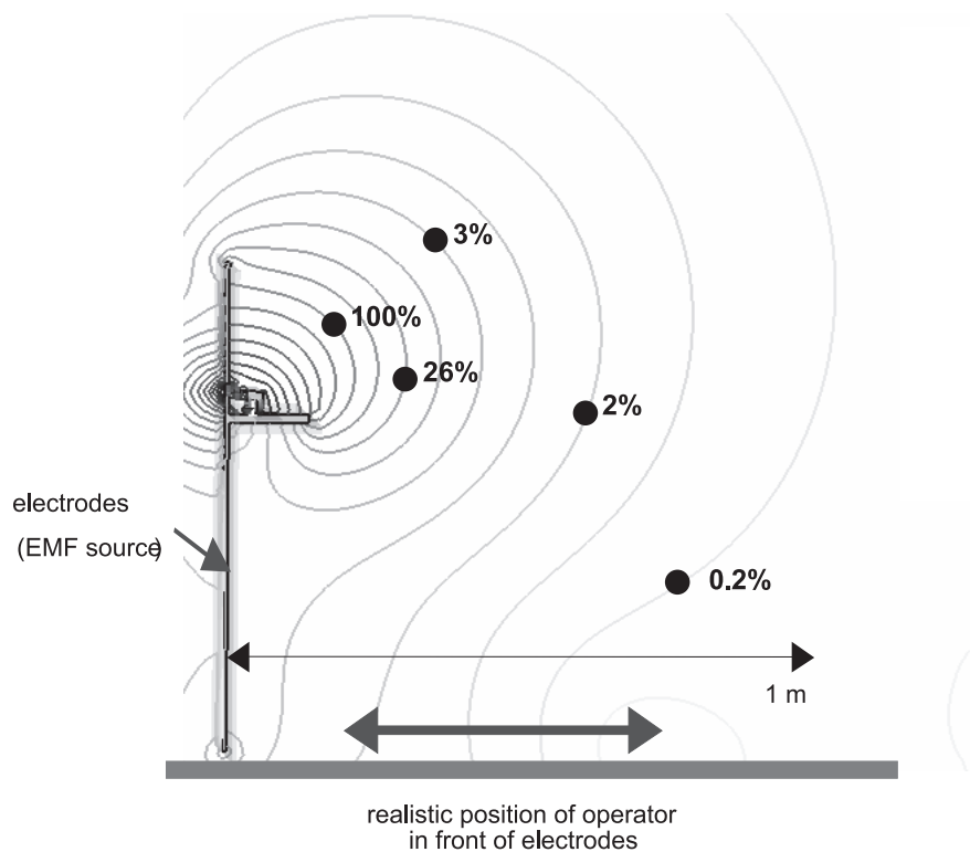
Figure 9. Examples of spatial distribution of electric field strength in front of a plastic sealer; the height of the electrode: 80 cm [7]. Notes. EMF—electromagnetic fields.
