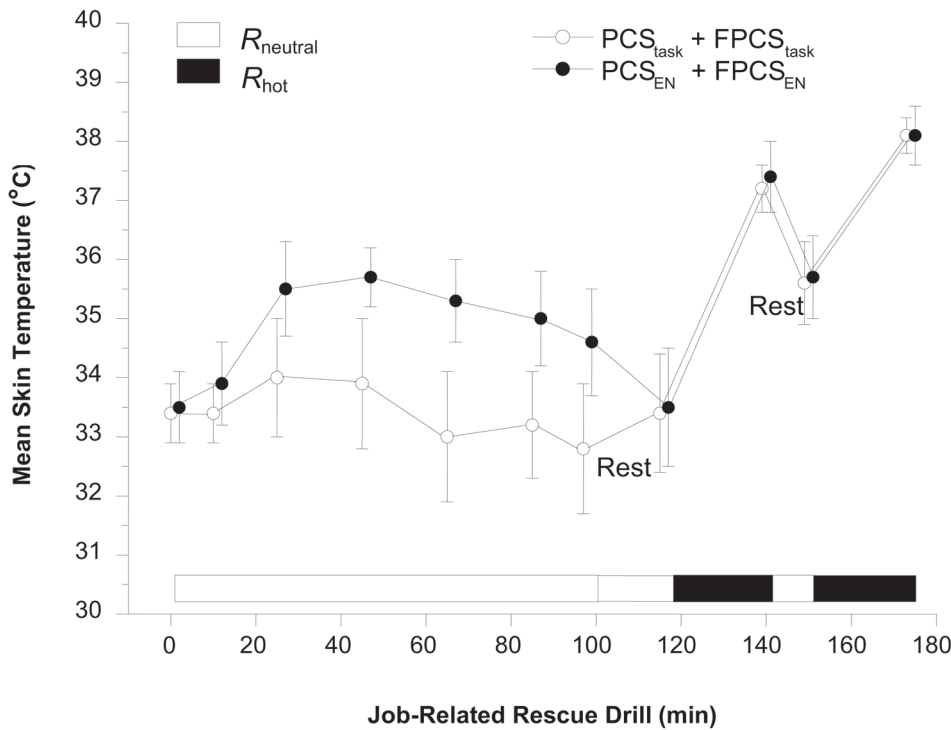
Figure 5. Average time courses for mean skin temperature ( N = 23 ) during a job-related rescue drill while PCS_{task} and PCS_{EN} in R_{neutral} and FPCS_{task} and FPCS_{EN} in R_{hot} were worn. Notes. R_{neutral} —22–25 °C/45–50% RH, R_{hot} —45 °C/35% RH; RH—relative humidity; ○—task-fitted protective clothing system, PCS_{task} , and task-fitted fire-protective clothing system, FPCS_{task} ; ●—protective clothing system that meets the requirements of Standard No. EN 469:2005 [1], PCS_{EN} , and fire-protective clothing system that meets the requirements of Standard No. EN 469:2005 [1], FPCS_{EN} .
