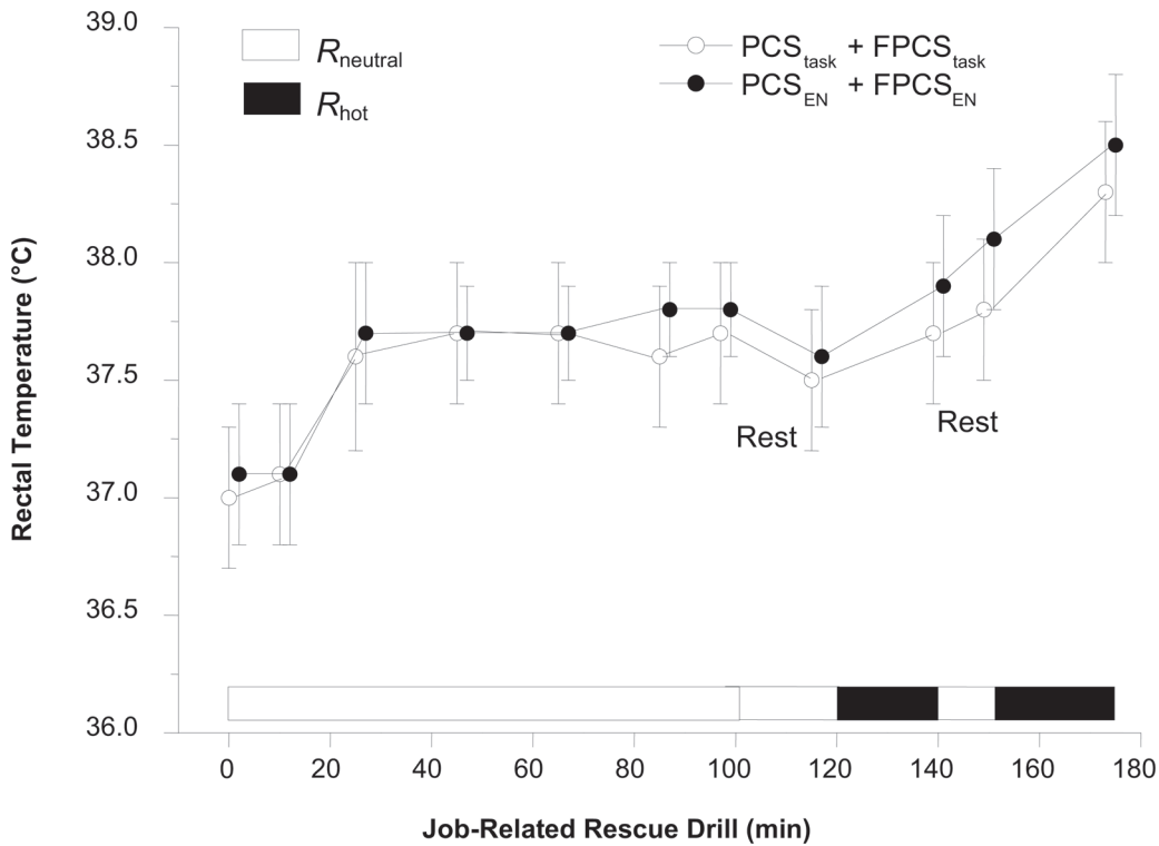
Figure 3. Time courses for mean rectal temperature ( N = 23 ) during a job-related rescue drill while PCS_{task} and PCS_{EN} in R_{neutral} and FPCS_{task} and FPCS_{EN} in R_{hot} were worn. Notes. R_{neutral} —22–25 °C/45–50% RH, R_{hot} —45 °C/35% RH; RH—relative humidity; ○—task-fitted protective clothing system, PCS_{task} , and task-fitted fire-protective clothing system, FPCS_{task} ; ●—protective clothing system that meets the requirements of Standard No. EN 469:2005 [1], PCS_{EN} , and fire-protective clothing system that meets the requirements of Standard No. EN 469:2005 [1], FPCS_{EN} .
