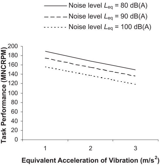
Figure 6. Relationship between task performance and equivalent acceleration of vibration at different noise levels for both male and female operators. Notes. MNC RPM—mean number of characters read per minute.
